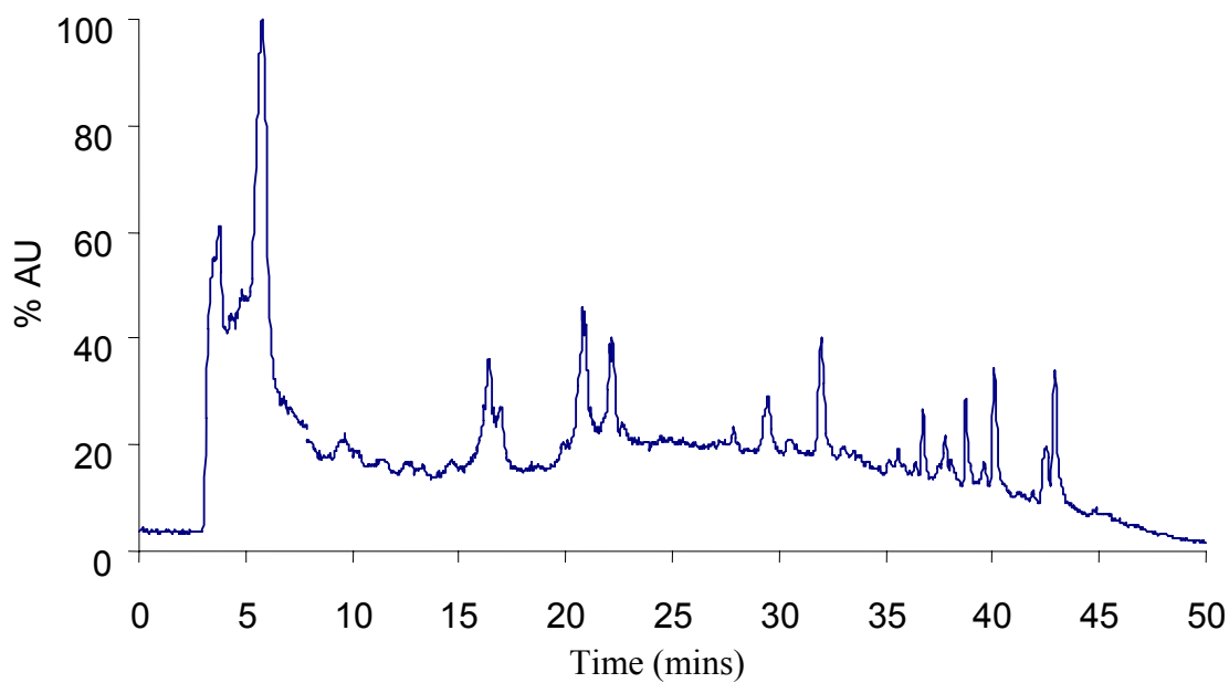
Figure 36. Chromatogram with MS detection of the degraded lignin showing numerous peaks
