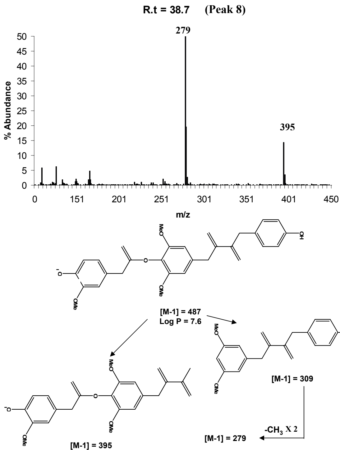
Figure 45. Mass fragmentation pattern of a \beta -O-4 and \beta - \beta linked trimer at retention time 38.7
