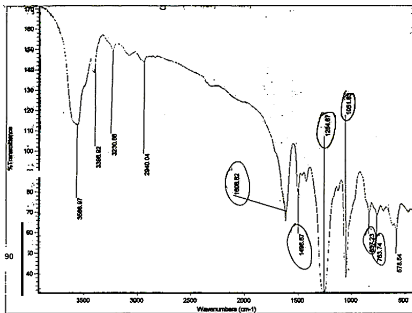
Figure 17: IR spectrum of the sulfated polymer showing presence of aromatic region, presence of acidic and hydroxyl groups but absence of carbonyl groups
